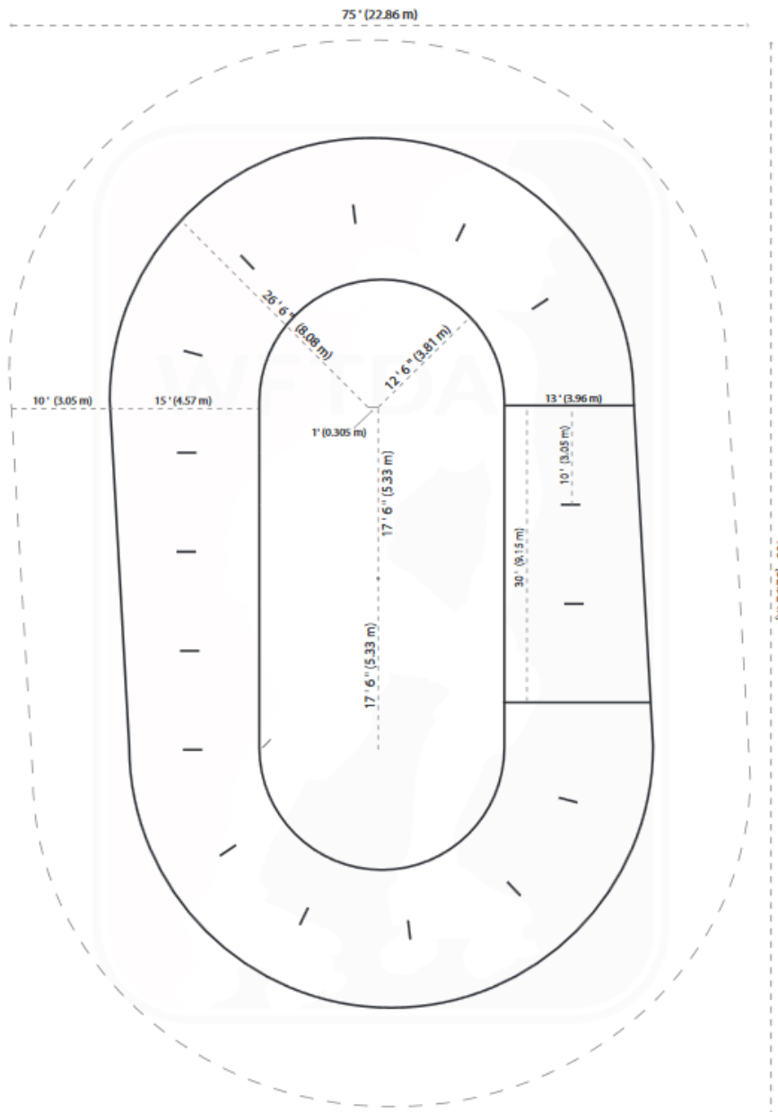
Fig. 12 - WFTDA Track Specifications
